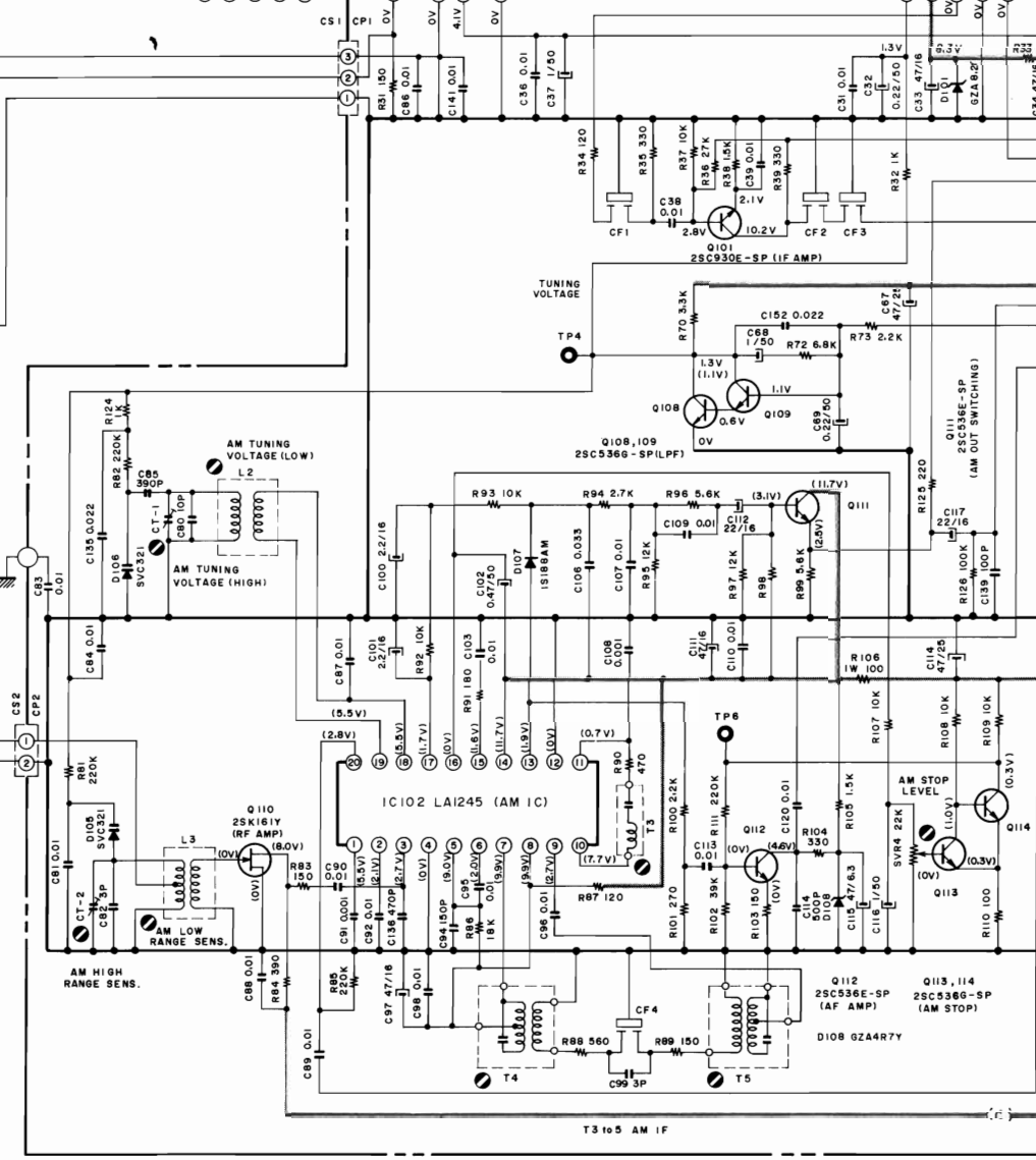
TUNER PCB R4174807
